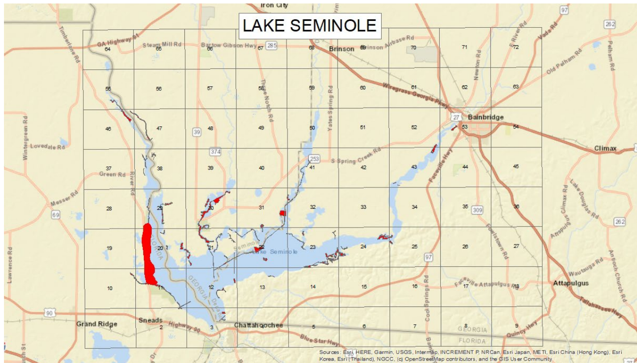
Figure 3: Map Plates
